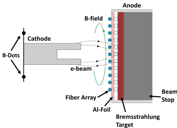
FIG. 2. Four B-dots are placed 90° apart behind the cathode to measure the beam current and the current due to back streaming ions from the anode surface plasma. The 11-fiber array images the foil surface (filled circles) or the anode target (unfilled circles), depending on the diode configuration.
